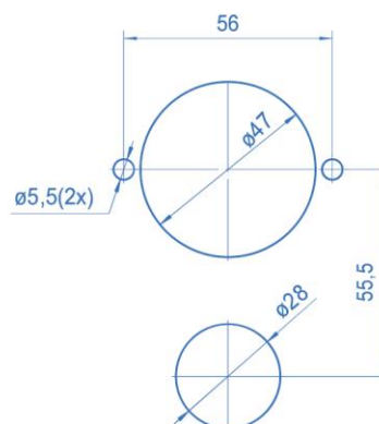
Bore template for installation
