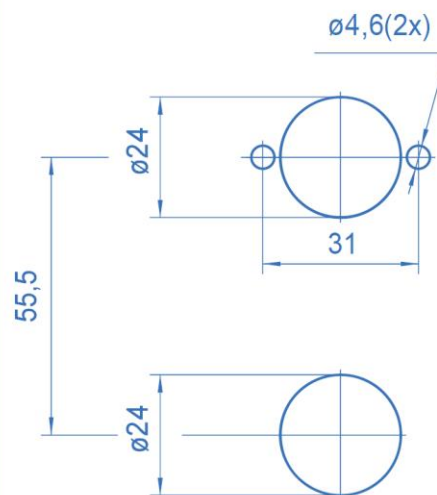
Bore template for installation
