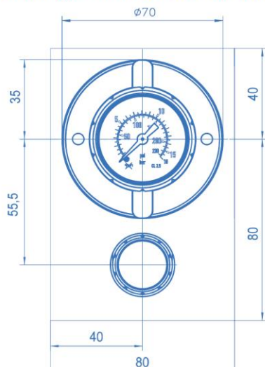
Front view with recommended modular dimensions
